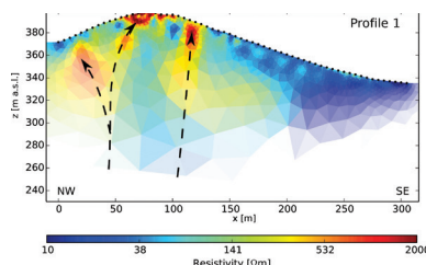
Two-dimensional inverted resistivity (electrical resistivity tomography) image of the Zebín Volcano along profile 1. The low-resistivity zones (up to approximately 100 \Omega\text{m} , blue and bluish colours) represent clay-rich sediments, whereas the high resistivity areas (approximately 300 \Omega\text{m} and more, red colours) represent coherent basic dikes. The possible magma feeder conduits/dikes are indicated by dashed arrows.
