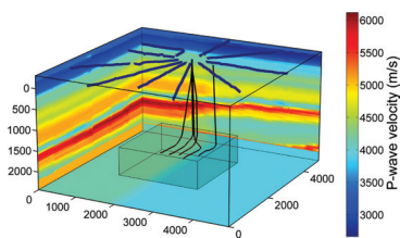
3D P-wave velocity model, wells and surface star-like monitoring array acquiring microseismic data during hydraulic fracturing in shale
