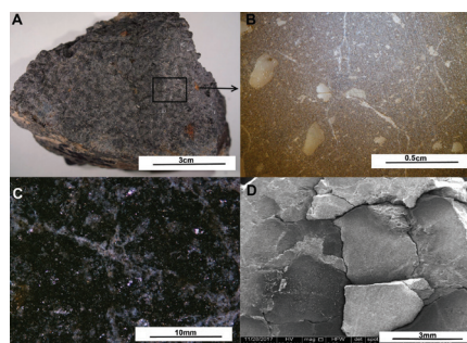
The sunburn effect of basalt from macro to micro scale. a – Macro photograph of the sample, spots are clearly visible; b – Macro photograph of capillary cracks and analcite minerals; taken by digital microscope Keyence VHX-5000; c – Spots and “white sun” under the optical microscope with plane-polarized light; d – Cracks captured by SEM.
