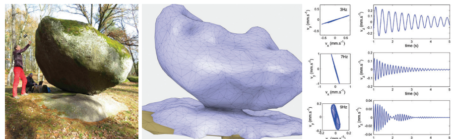
Left: Seismic measurements of the Hus Pulpit balanced rock; middle: its 3-D digital model created from 163 images using the Agisoft PhotoScan software; right: Partical motion analysis of the three fundamental eigenoscillations of the Hus Pulpit.
