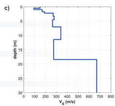
Velocity model retrieved from measurement and analysis of phase velocity
